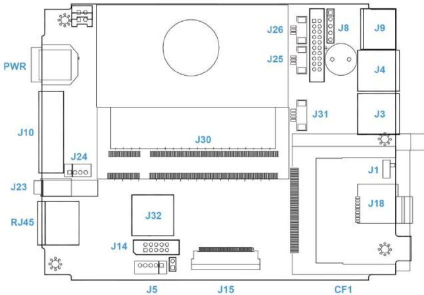
Fig 2-1 PEX CPU Board
