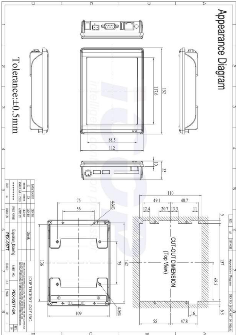
Fig 1-4 Product Dimension
