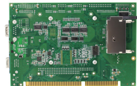
VDX2-6524-CF (Rear)
