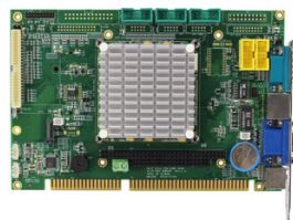
VDX2-6524-CF (Front)
