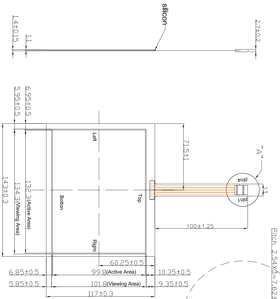
"A" DETAIL
