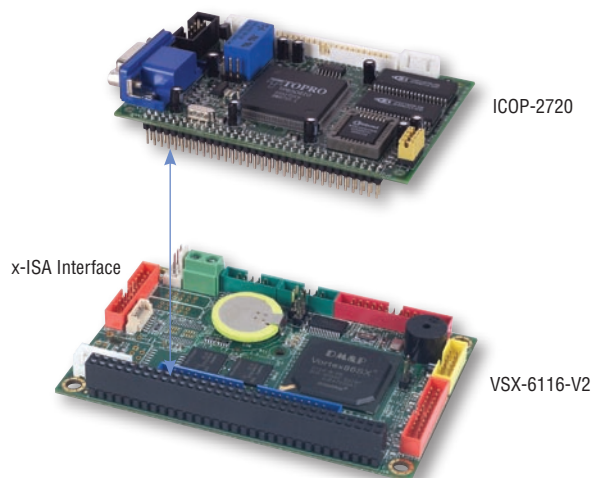
VGA function support via x-ISA interface
